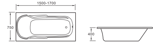
TR-C0301 Size:1700X750X400mm TR-C0302 Size:1600X750X400mm TR-C0303 Size:1500X750X400mm
