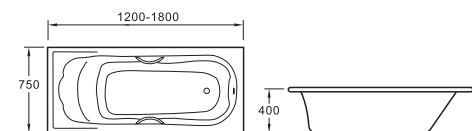
TR-C1183 Size: 1800X900X400mm TR-C1184 Size: 1700X750X400mm TR-C1185 Size: 1600X750X400mm TR-C1186 Size: 1500X750X400mm TR-C1187 Size: 1500X700X400mm TR-C1188 Size: 1400X750X400mm TR-C1189 Size: 1200X750X400mm
