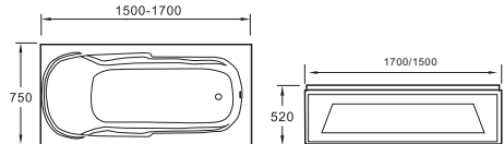
TS-0031 Size:1700X750X520mm TS-0032 Size:1500X750X520mm
